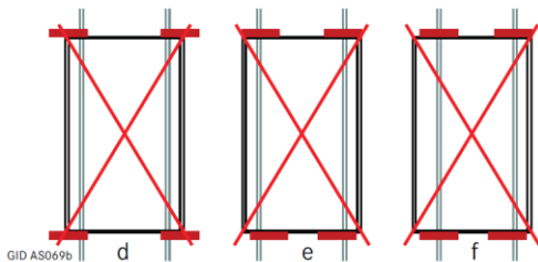
Fig. 7 Impermissible clamp arrangements (2) d : Protruding clamps, e : Opposing clamps have different distances to the PV module corners, f : Asymmetrical clamps on the short sides.
