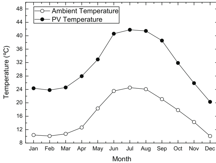
Fig. 5. Monthly averaged hourly ambient air and PV module temperature measured during daylight hours for 2007.
