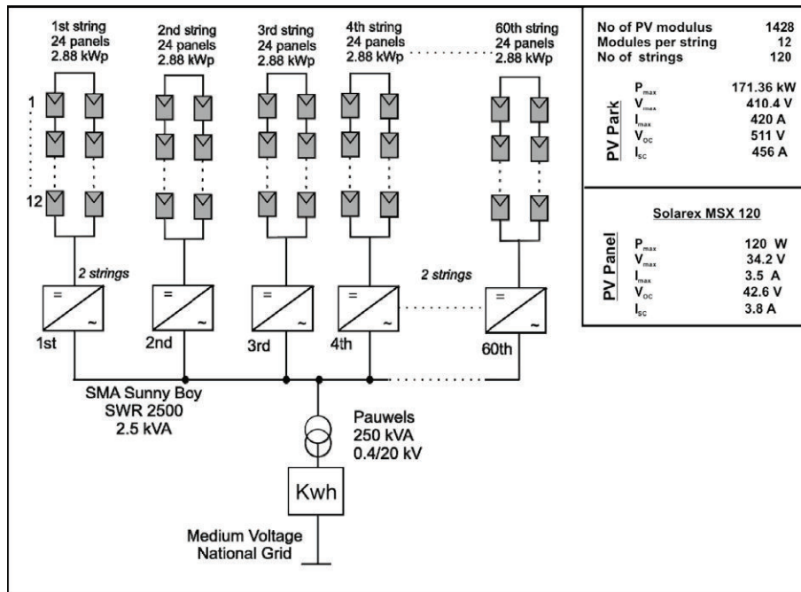
Fig. 2. Schematic block circuit diagram of the PV system.
