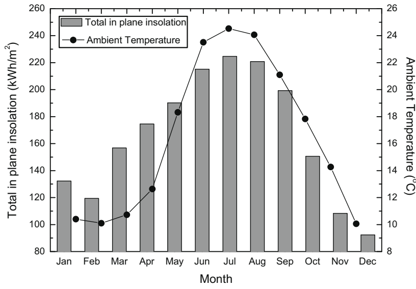
Fig. 3. Monthly averaged total in-plane insolation and ambient temperature averaged during the daytime hours over the year 2007.
