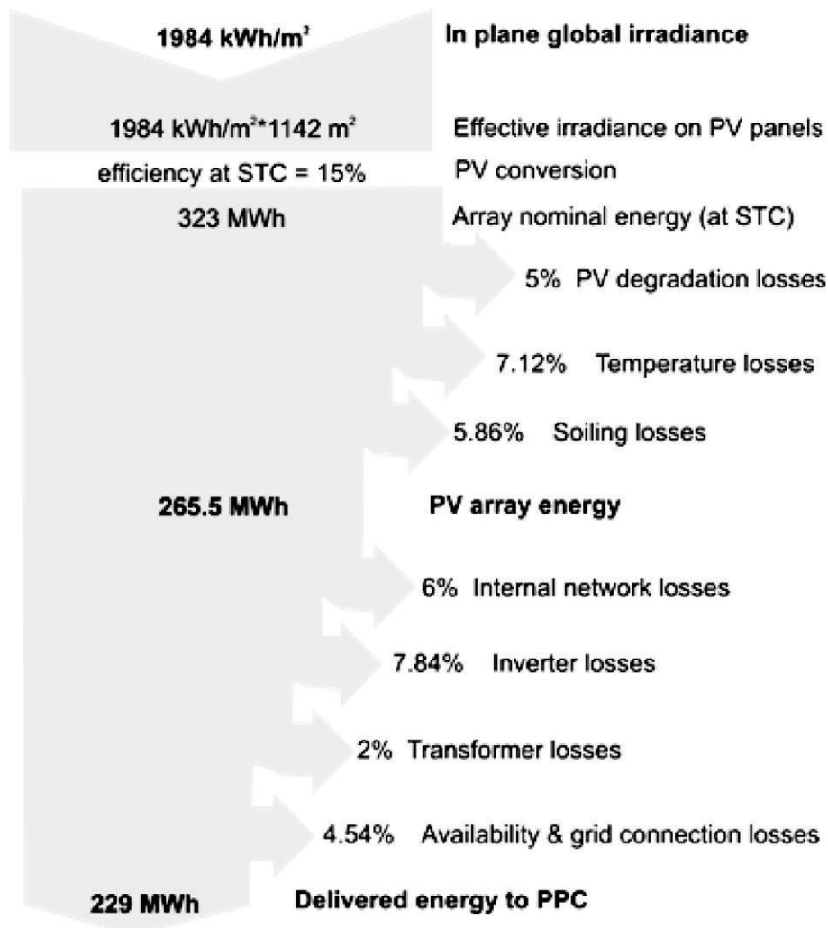
Fig. 7. Sankey diagram of estimated losses in the PV park, the parameters in bold are derived from the real measurements raw data analysis.
