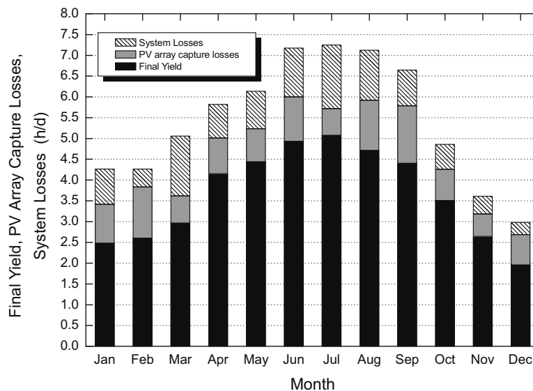
Fig. 4. Monthly averaged daily final yield, PV array capture losses and system losses.
